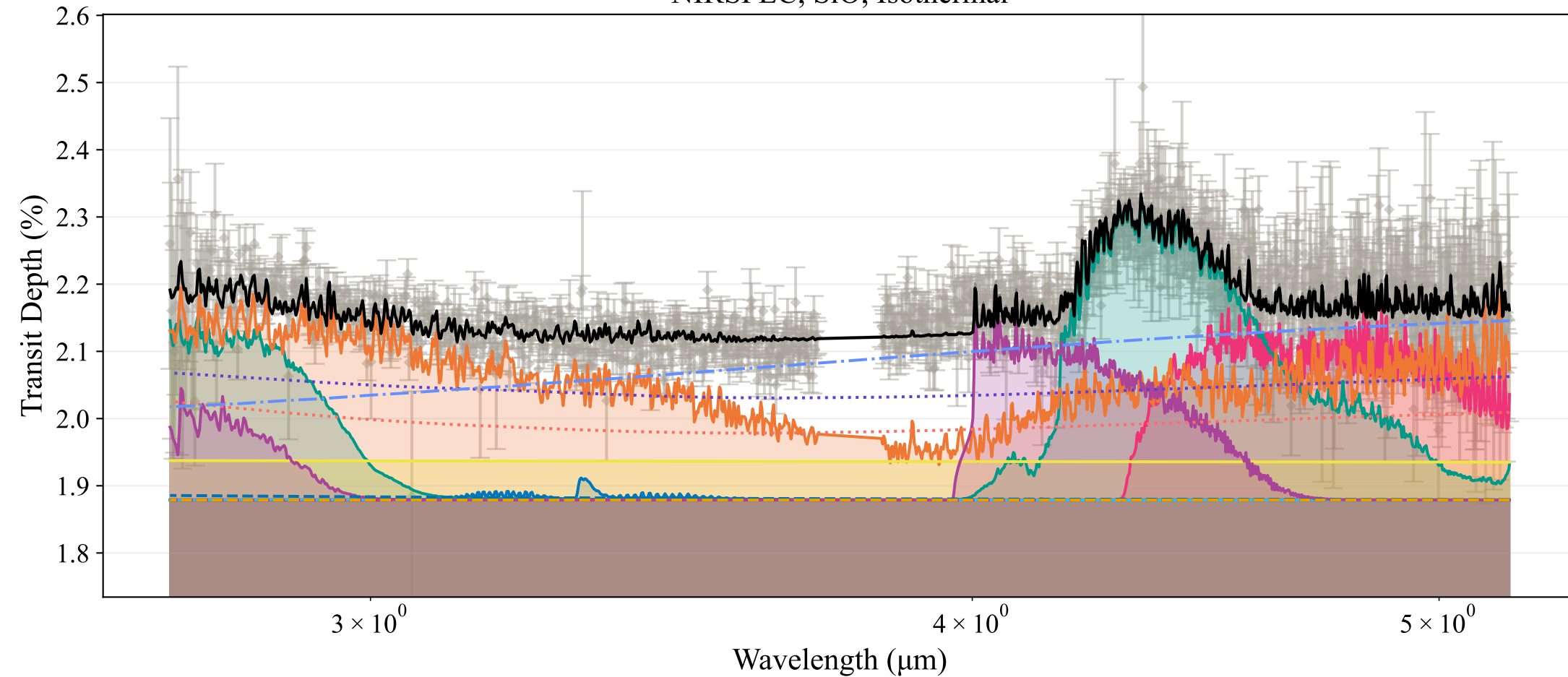
NIRSPEC, SiO, Isothermal
